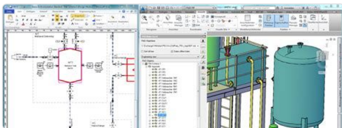
From P&ID to 3D model – project, tagging and catalogs from one source
